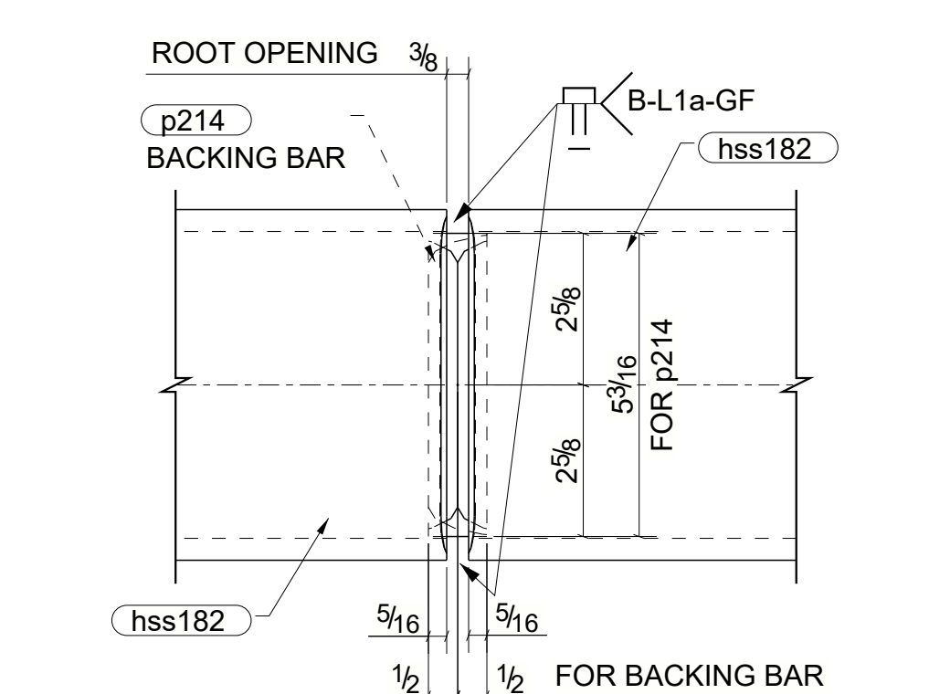
DETAIL-A OTHERS NOT SHOWN FOR CLARITY
