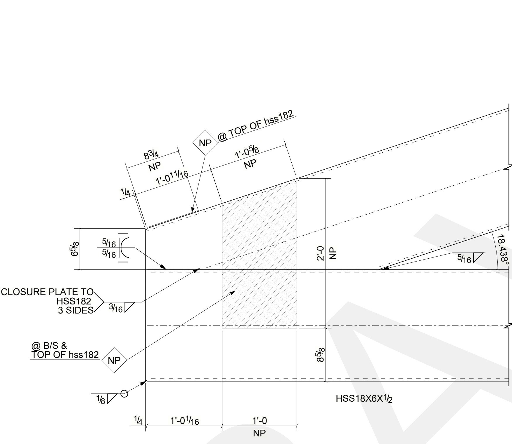
DETAIL-C OTHERS NOT SHOWN FOR CLARITY
