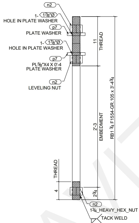
40-ANCHOR ROD-1001AB1
