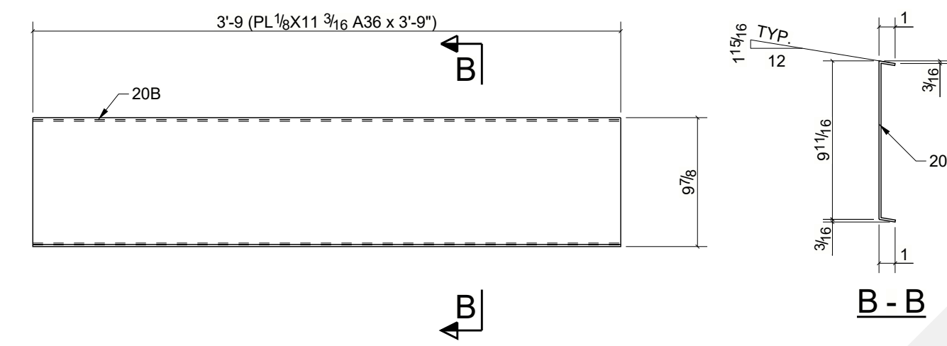
1 ~ TREAD PLATE ~ 20B
