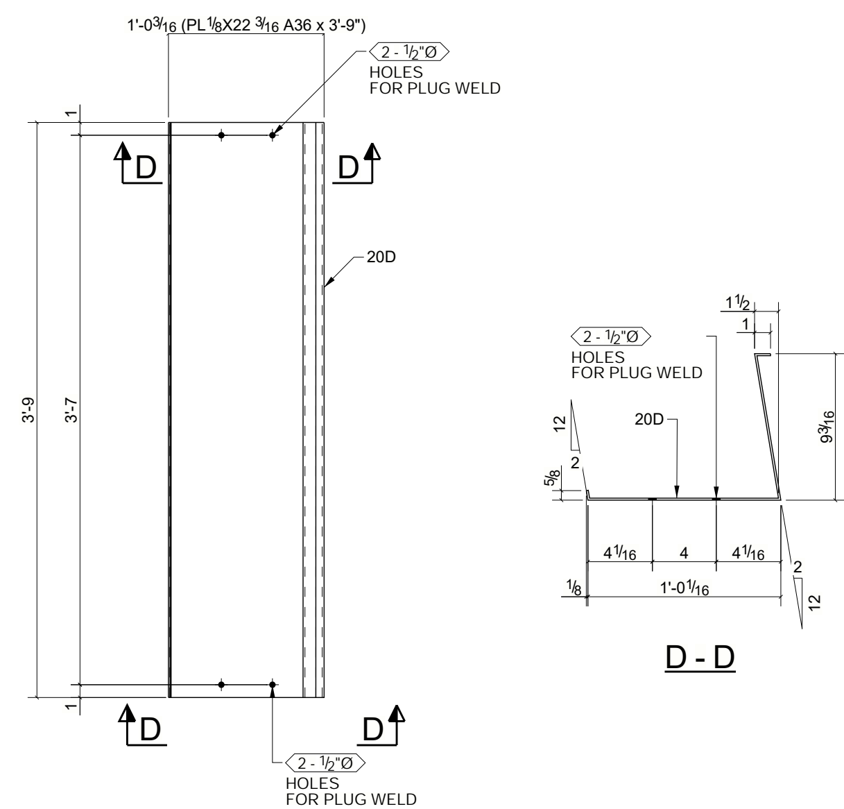
13 ~ TREAD PLATE ~ 20D
