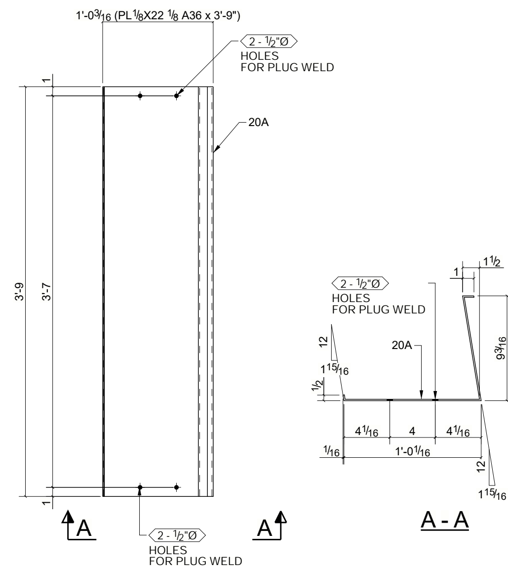
7 ~ TREAD PLATE ~ 20A
