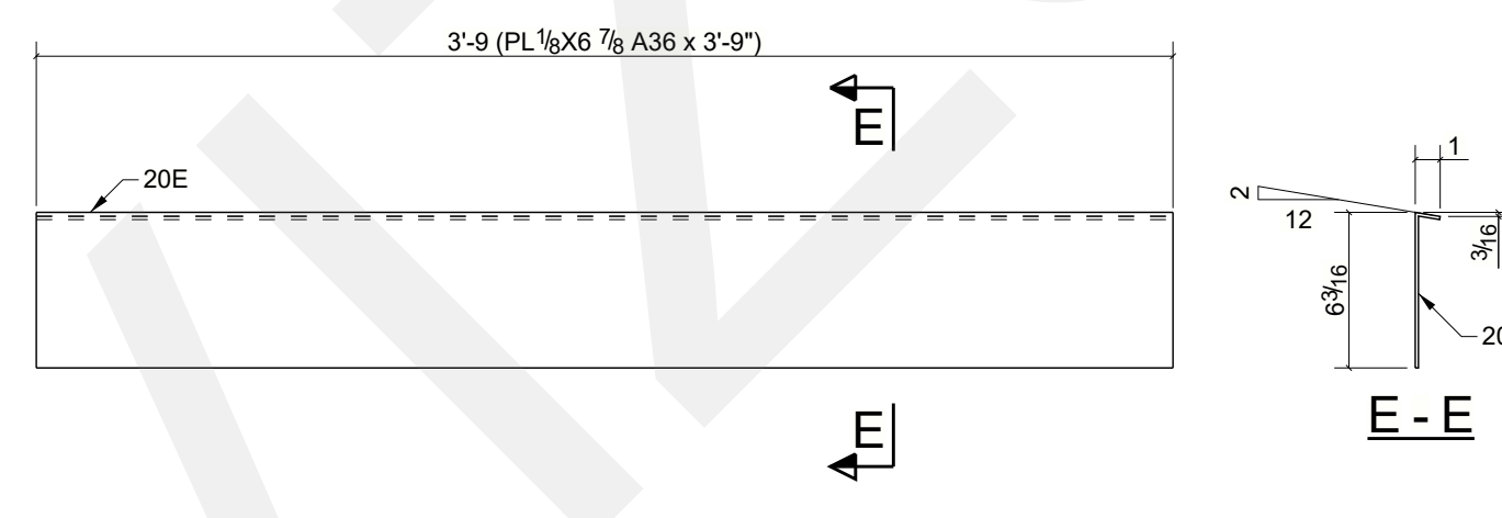
1 ~ TREAD PLATE ~ 20E
