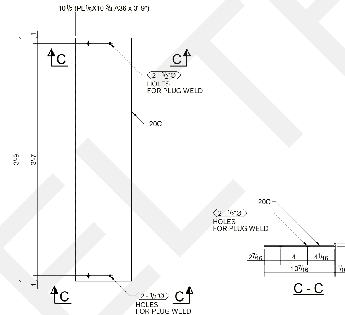
1 ~ TREAD PLATE ~ 20C
