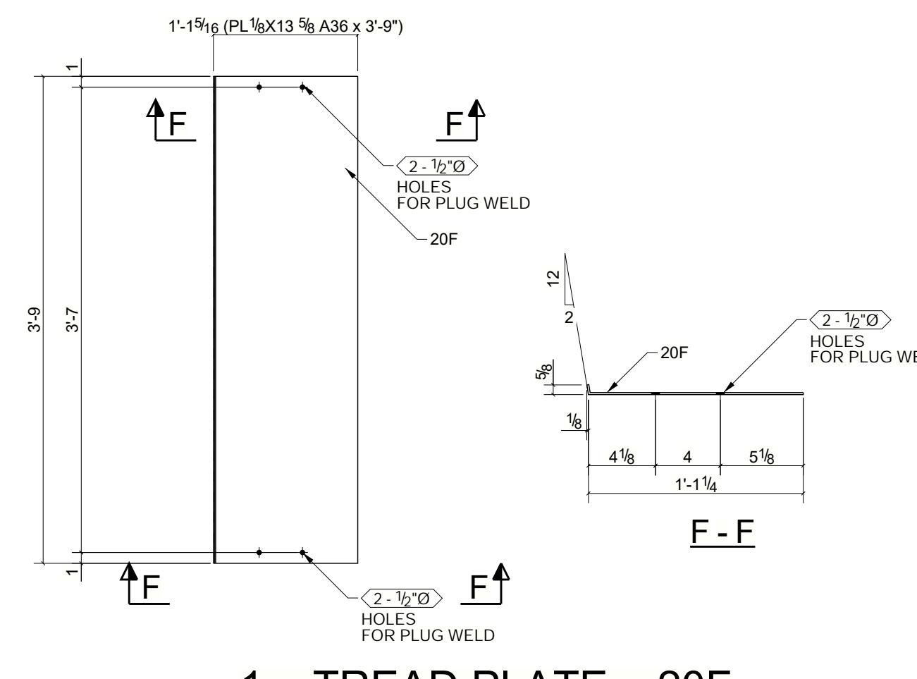
1 ~ TREAD PLATE ~ 20F
