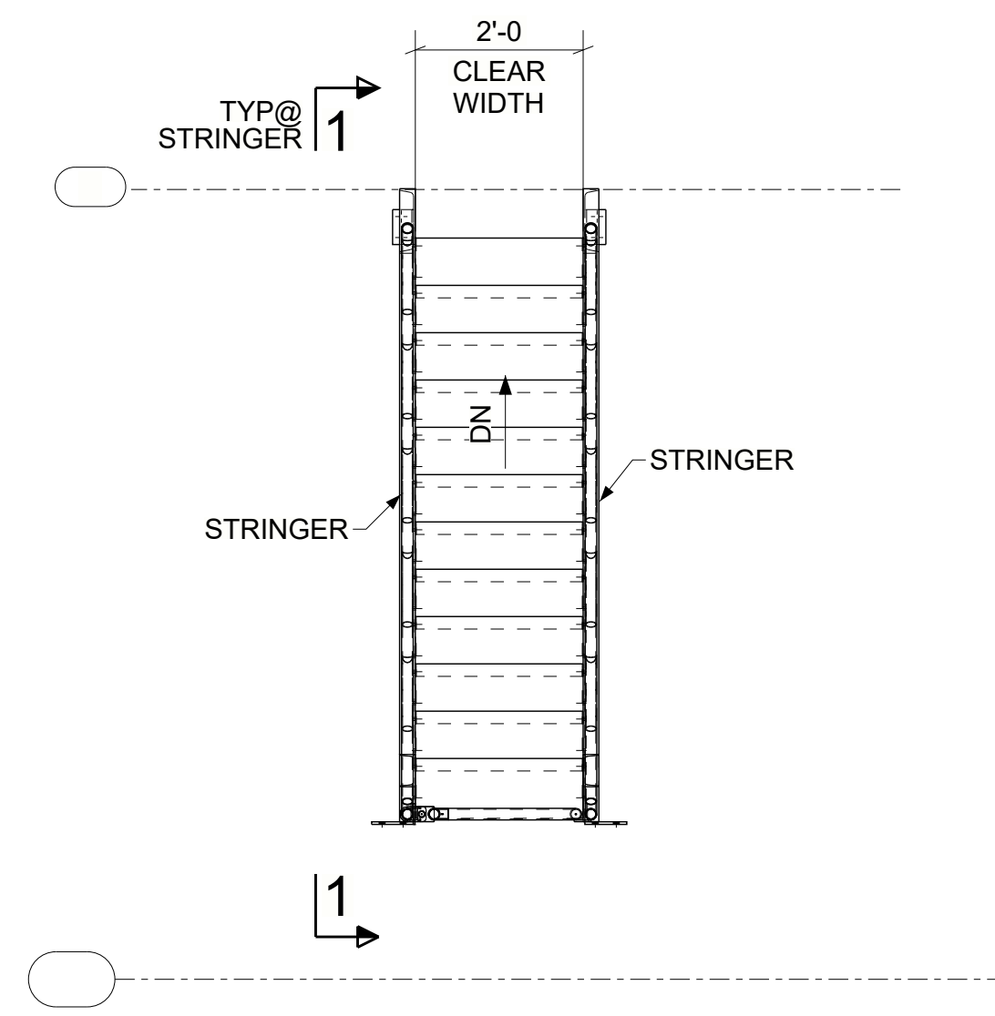
SHIP LADDER PLAN
